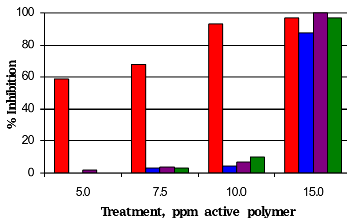
Figure 1: Calcium phosphate inhibition at 158°F (70°C) with a 400 ppm calcium hardness water.
